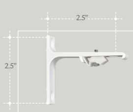
Single bracket TRB8143 - 39J7001 Brown TRB8143 - 90J7001 White
