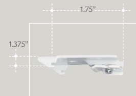
Ceiling bracket for motorized TRC8191 - 90J7001 White Note: cannot be used with fascia.
