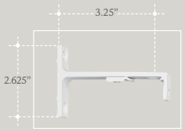
Single bracket for motorized TRB8190 - 90J7001 White
