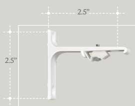
Single bracket TRB8143 - 39J7001 Brown TRB8143 - 90J7001 White
