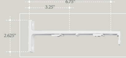
Double bracket for motorized TRB8189 - 90J7001 White Note: can also be used as single extension bracket.
