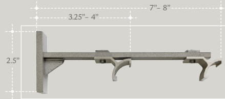
Adjustable double bracket TRB8114 - select finish Note: can also be used as single extension bracket.
