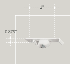
Ceiling bracket (track only) TCB8145 - 90J7001 White Note: cannot be used with fascia.
