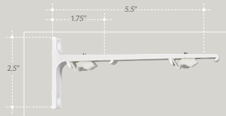
Double bracket TRB8144 - 39J7001 Brown TRB8144 - 90J7001 White Note: can also be used as single extension bracket.
