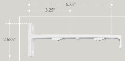
Double bracket for motorized TRB8189 - 90J7001 White Note: can also be used as single extension bracket.
