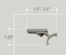
Adjustable ceiling bracket TCB8115 - select finish
