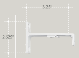
Single bracket for motorized TRB8190 - 90J7001 White
